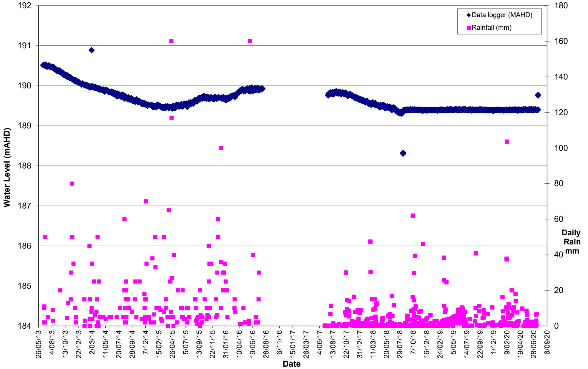
Figure HG-5: Monitoring Data Bore PFL2HitchMW1 (2013-2020)
