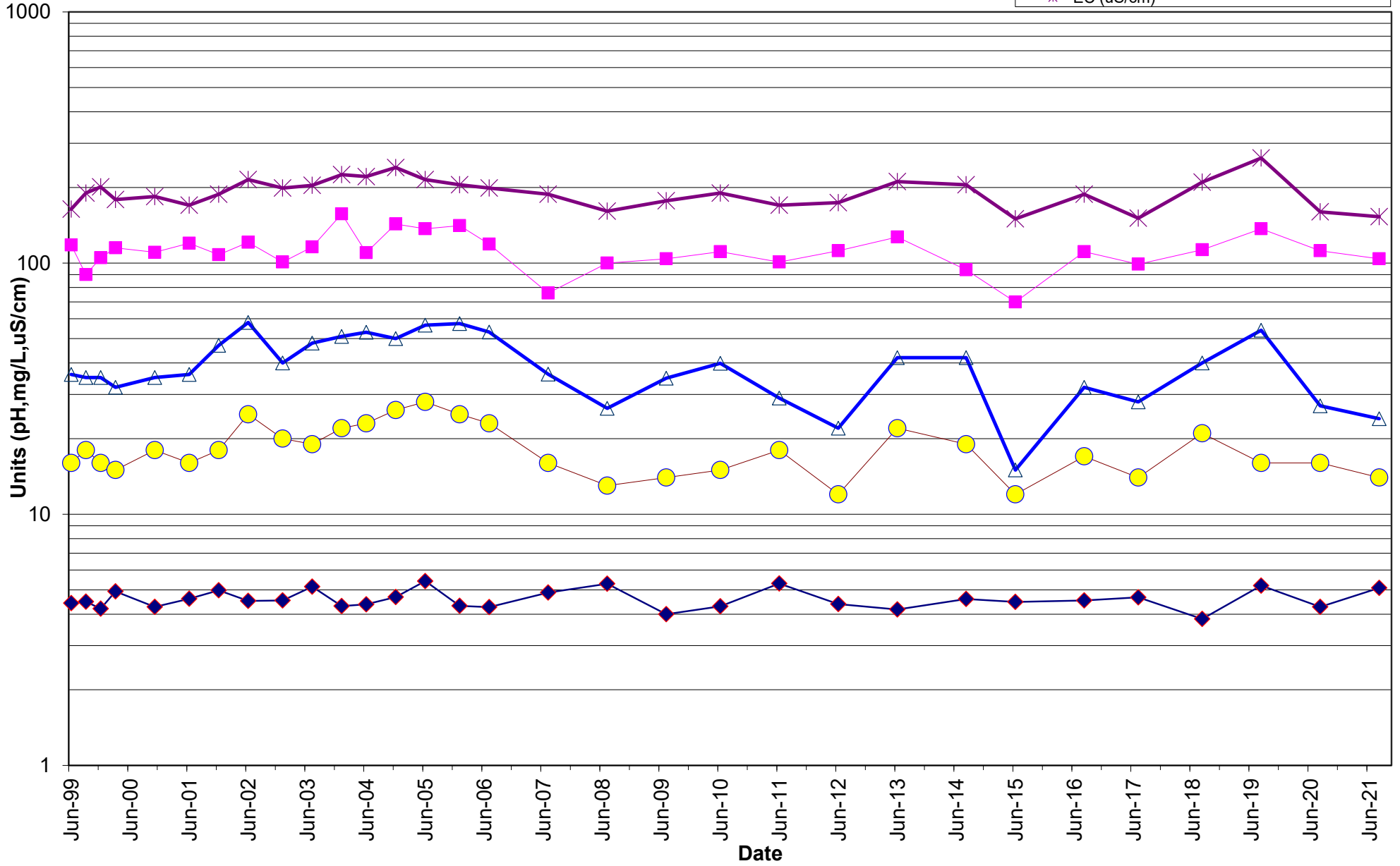
Graph -1: Groundwater Analytical Trends; Bore PF167MW1
