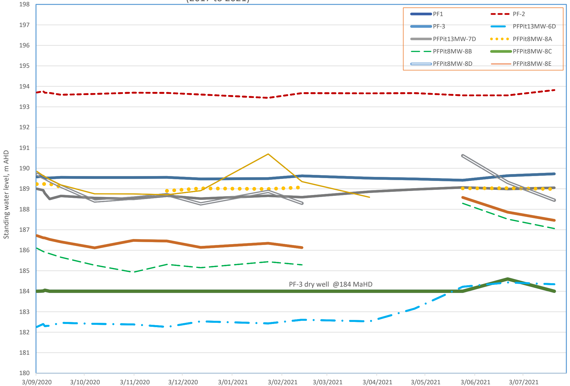
Figure HG-11A: Maroota; Monthly Groundwater Levels- Pits 8 & 13, & 4378 ONRd (2017 to 2021)
