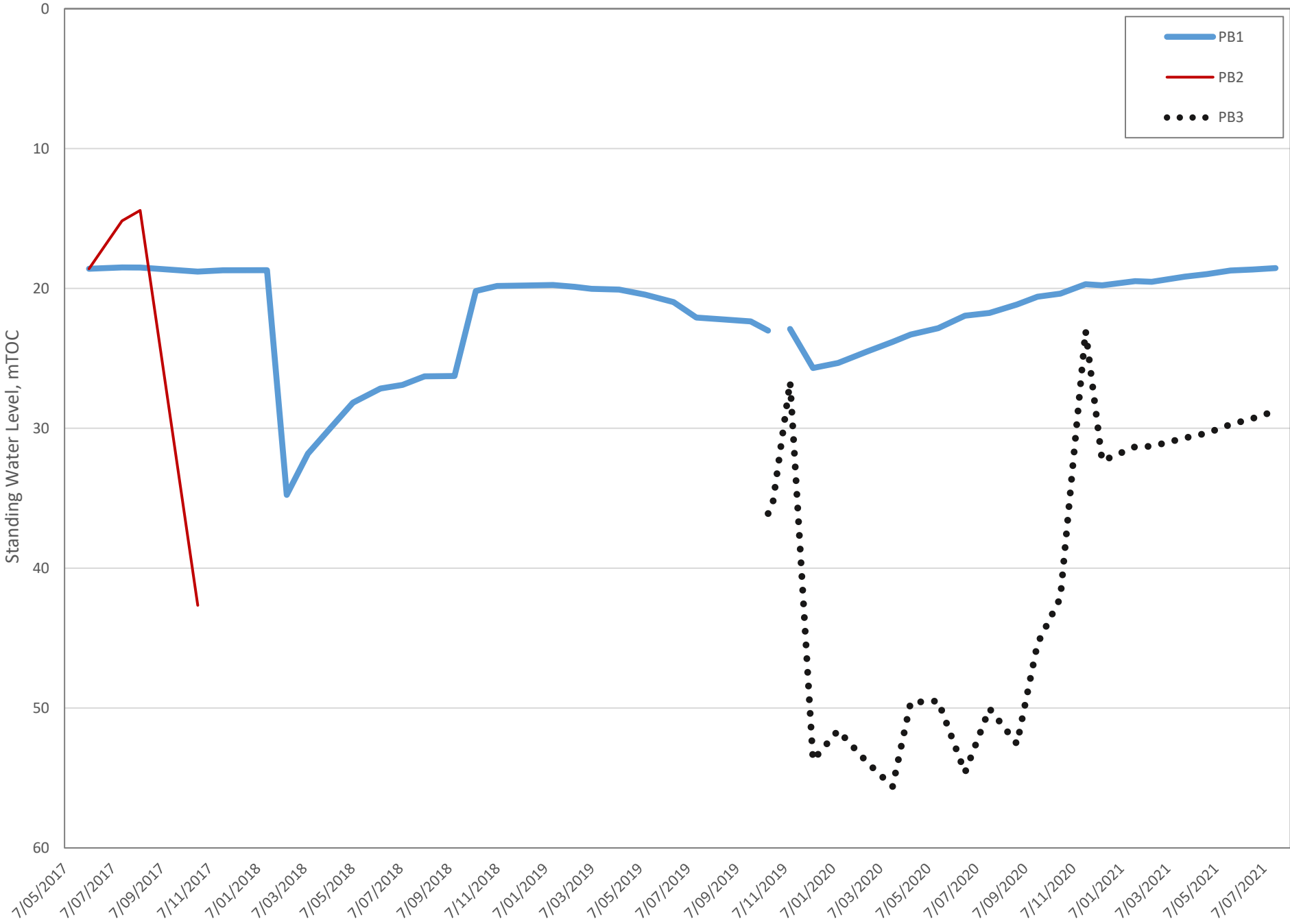
Figure HG-1: Manual Water Level Gauging at Lot 198 Wells (PB1, PB2, PB3), 2017 to 2021
