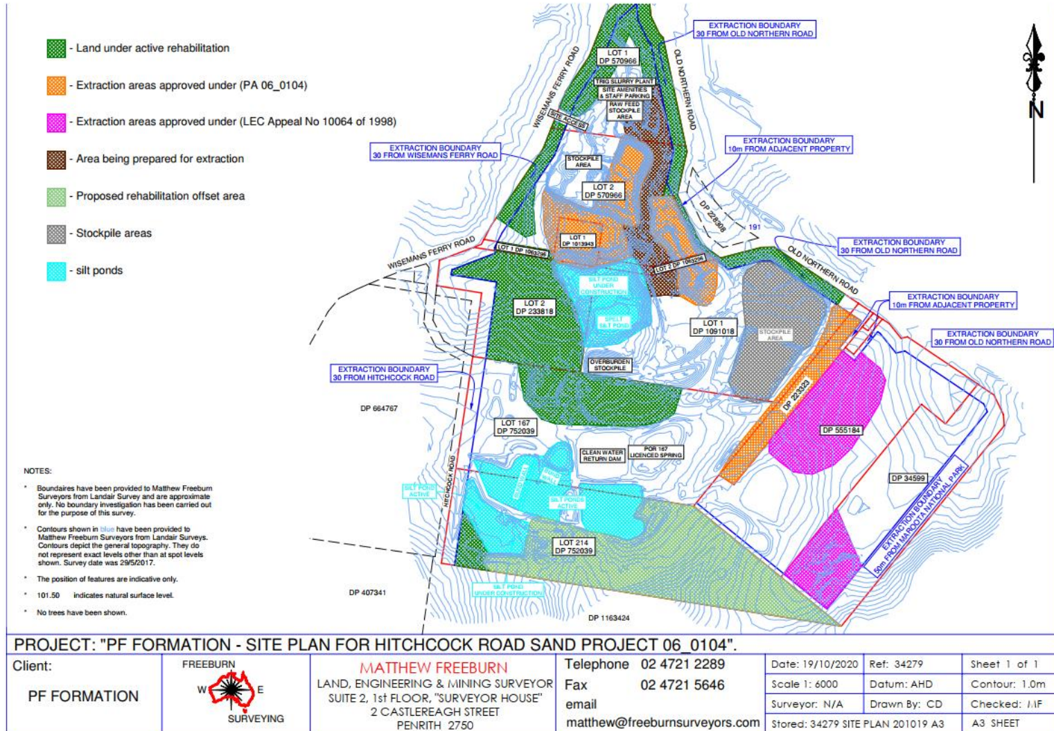
Figure 4. Current site plan November 2024
