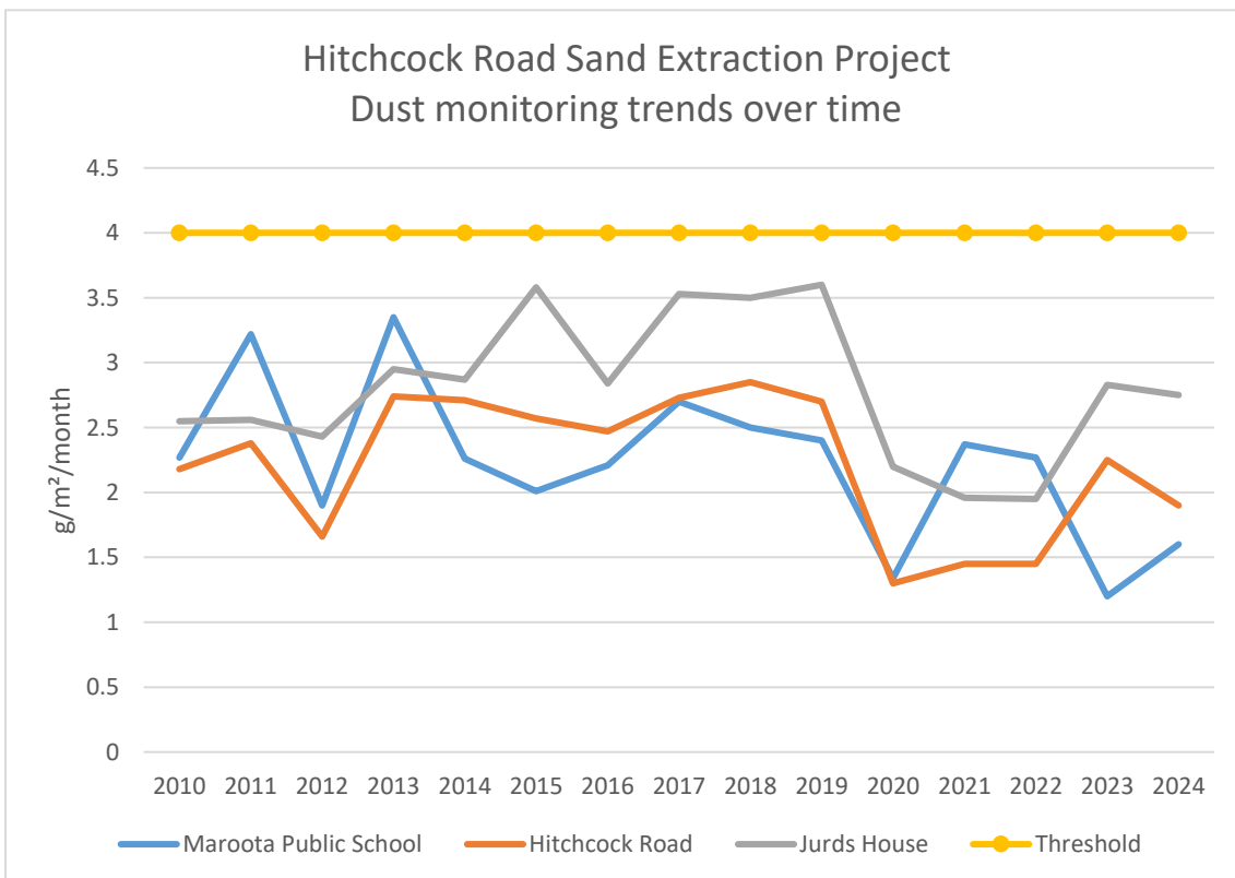
Chart 6. Dust monitoring trends over time – Insoluble Solids
