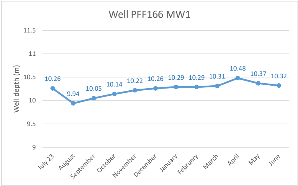
Chart 6. Ground water depth at monitoring bore 166MW1
