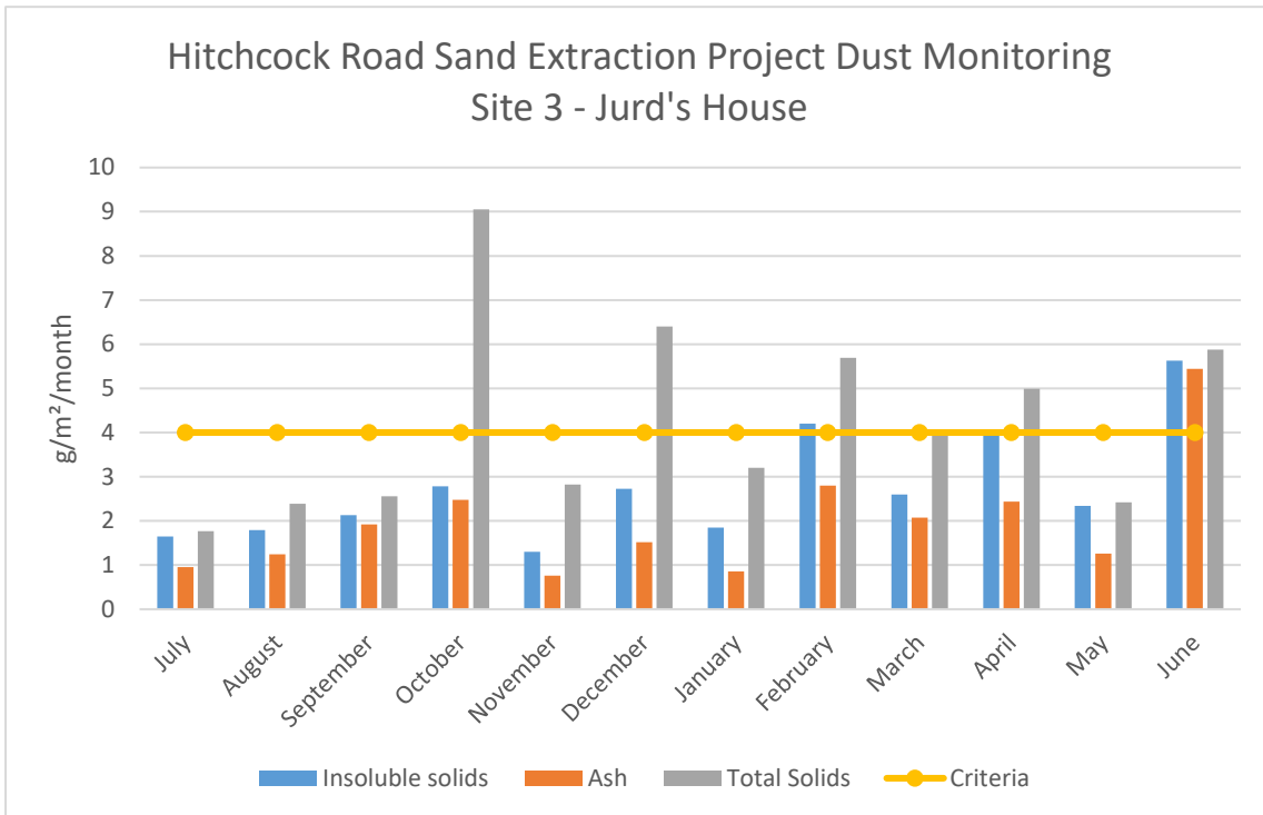
Chart 5. Dust monitoring results at Site 3 – Jurd’s House
