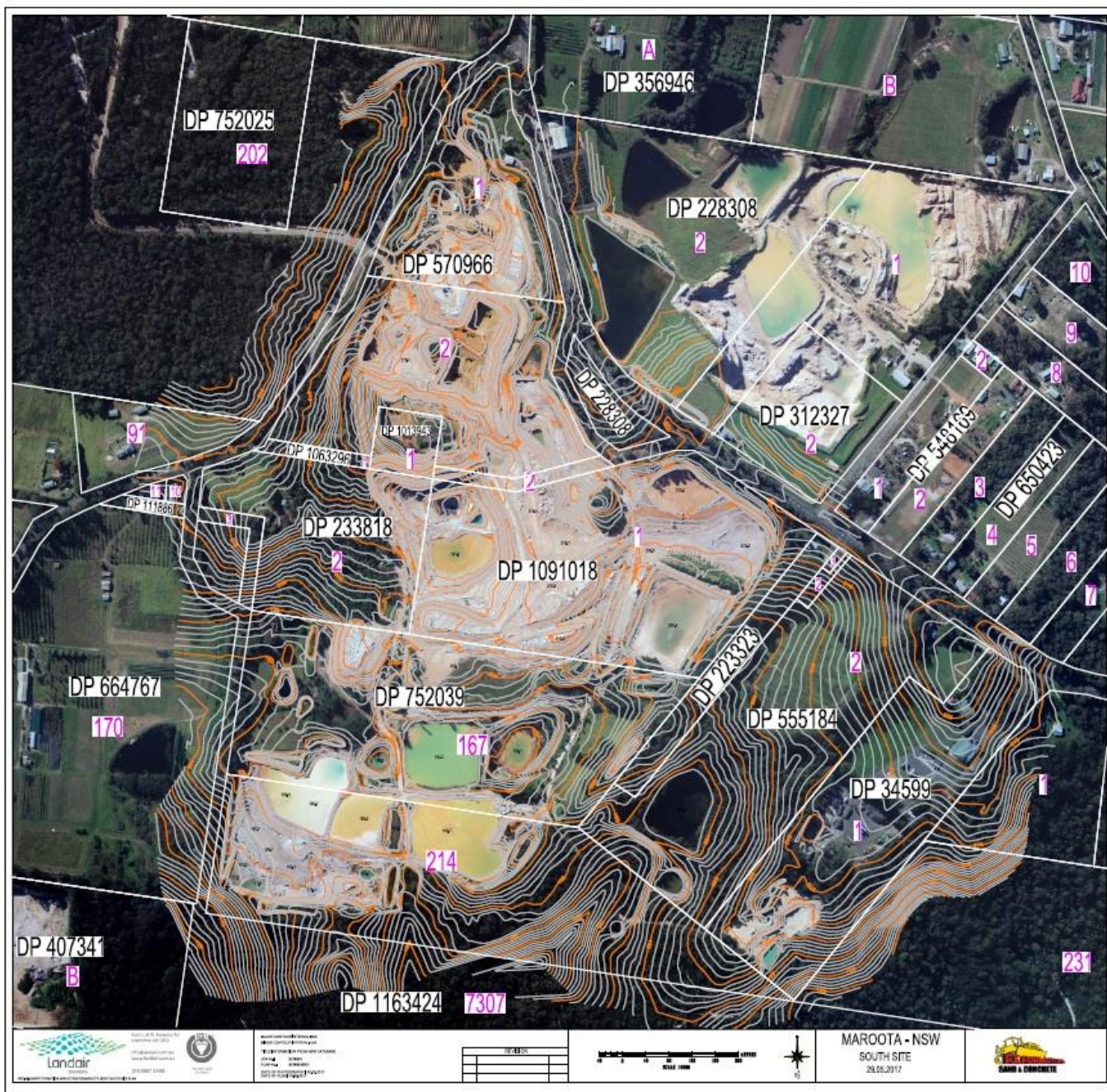
Figure 3. Contour map of lots within the Hitchcock Road Sand Extraction Project taken 2017
