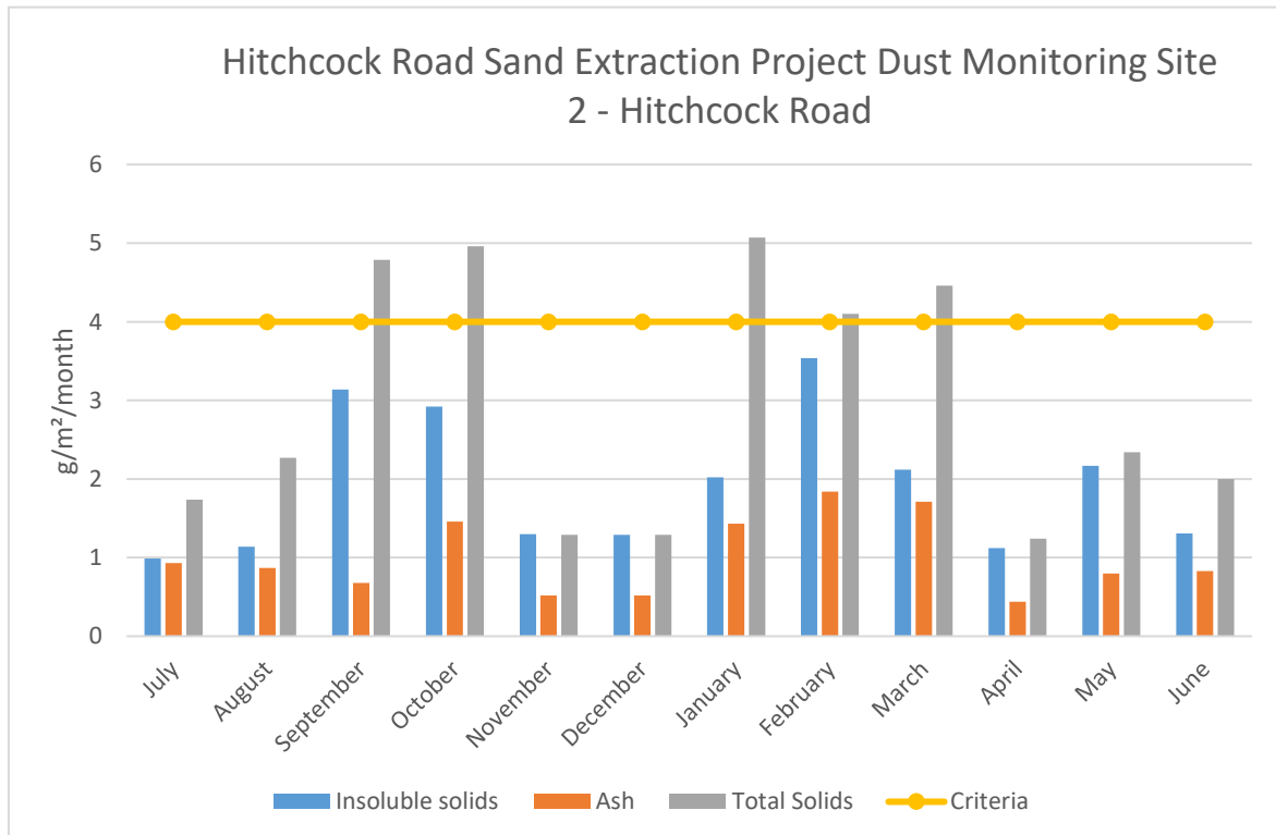
Chart 4. Dust monitoring results at site 2 – Hitchcock Road
