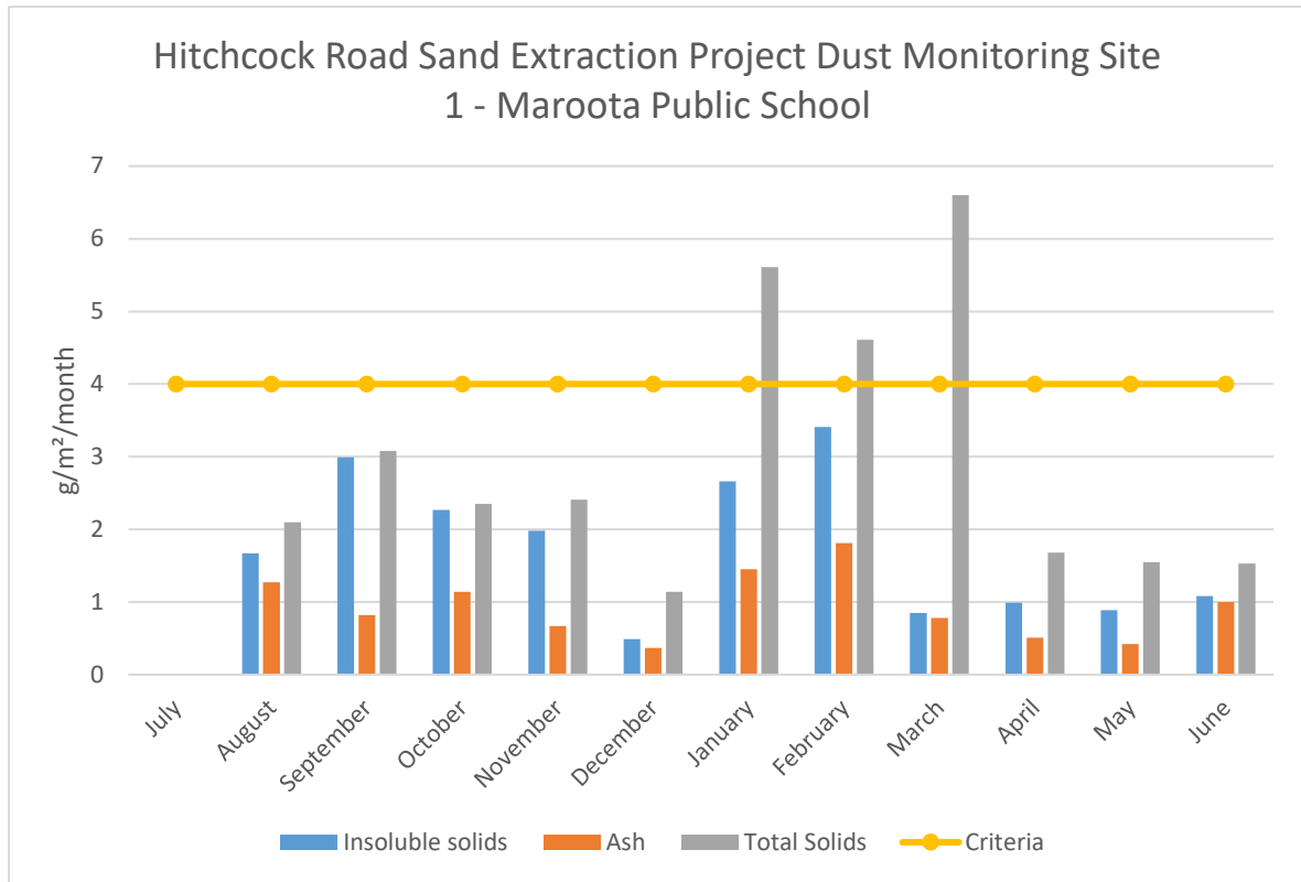
Chart 3. Dust monitoring results at Site 1 – Maroota Public School
