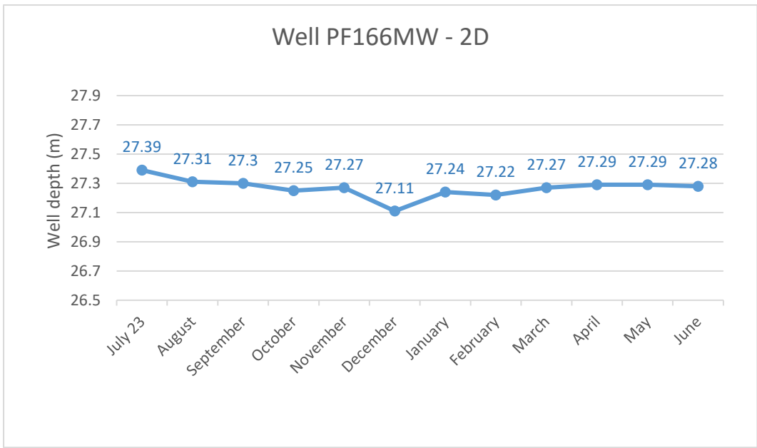
Chart 7. Ground water depth at monitoring bore 166MW-2D
