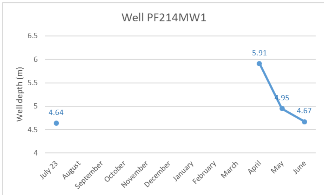
Chart 13. Ground water depth at monitoring bore 214MW1 (Access restricted during Aug-Apr)
