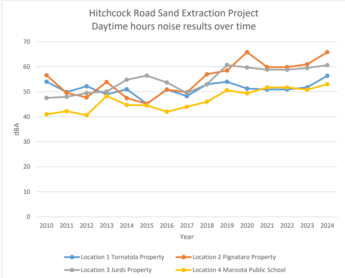
Chart 1. Daytime noise result trends over time
