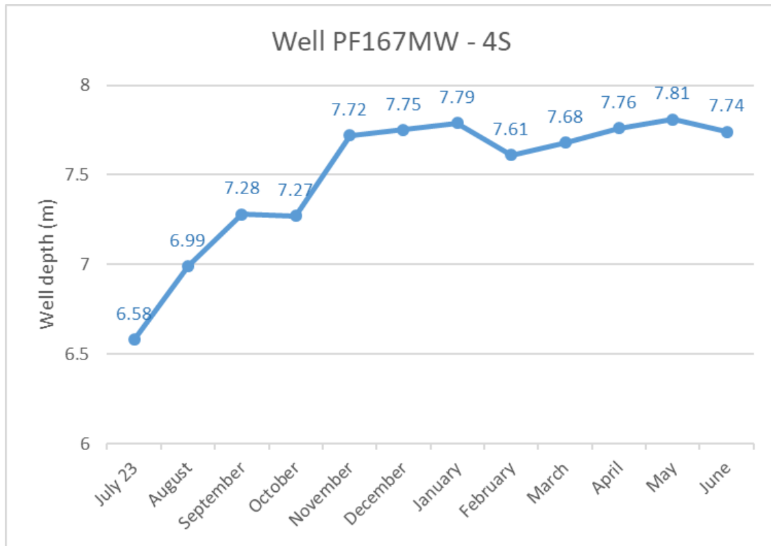
Chart 12. Ground water depth at monitoring bore 167MW-4S (Access restricted during Jul-Oct)
