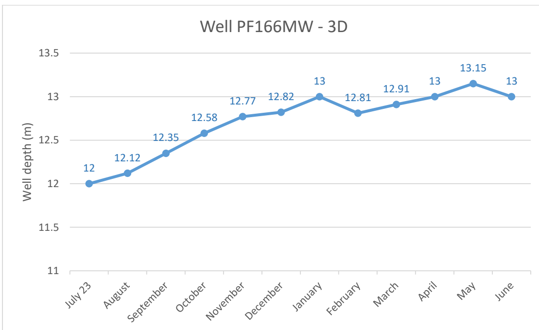
Chart 9. Ground water depth at monitoring bore 166MW-3D
