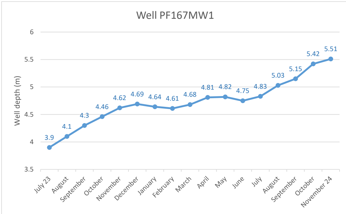
Chart 10. Ground water depth at monitoring bore 167MW1
