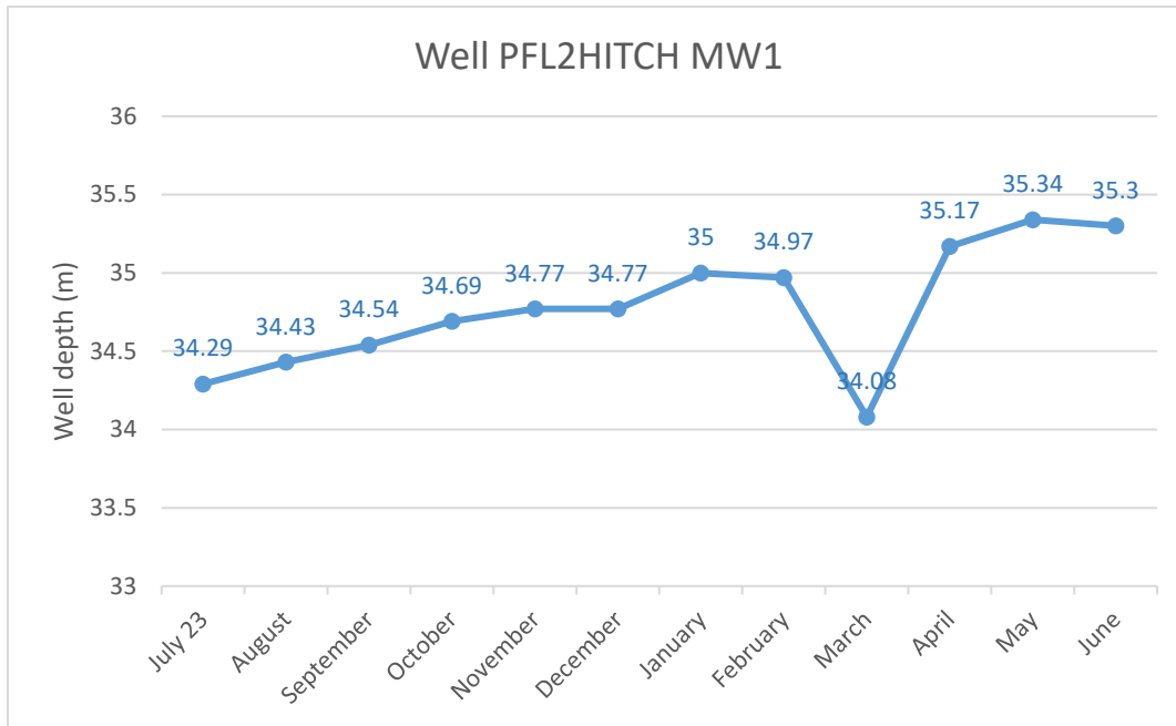
Chart 14. Ground water depth at monitoring bore HitchMW1 (Access restricted during August)
